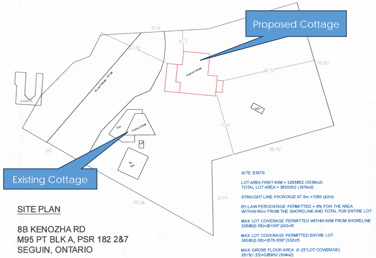
Figure 2: Site Sketch
